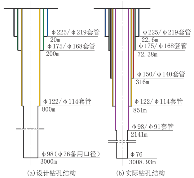
图2 ZK16508 孔钻孔结构 Fig.2 Drilling structure of ZK16508
